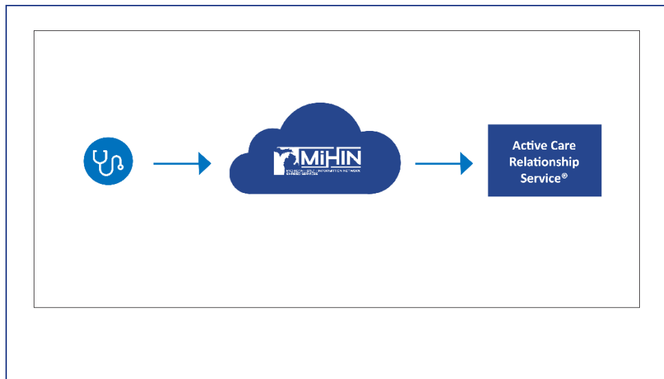
Figure 4. Manage ACRS
